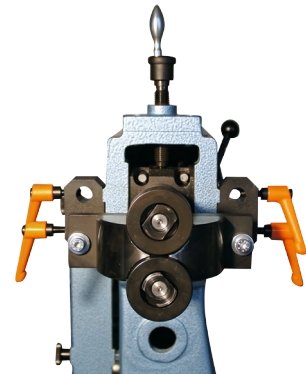
T-piece guide for inner cut-out
