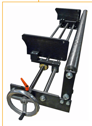
Infinitely adjustable sheet guidance with spindle, 0 - 1250 mm
