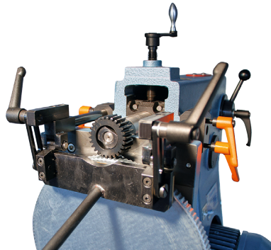
Turning and draw-in slide
