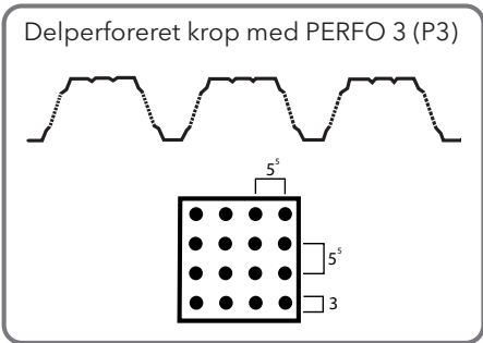
Perforeringsgrad: 23,4 %
